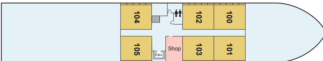
Main Deck
